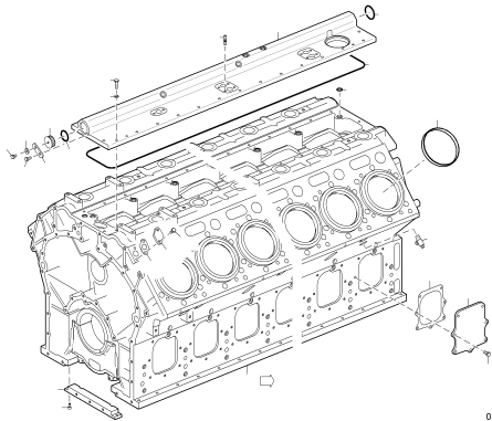
CRANKCASE X00026310
