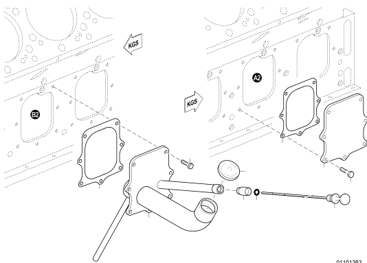
OIL FILLER NECK W OIL DIPSTICK, RGH XS594010.00099
